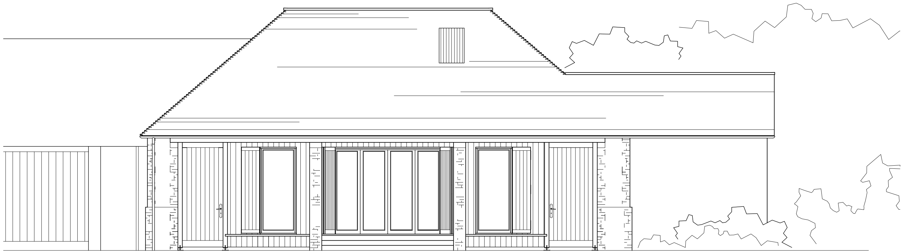
The Tractor Shed, Brighton Permaculture Trust Front ( east ) elevation, showing shutters open
