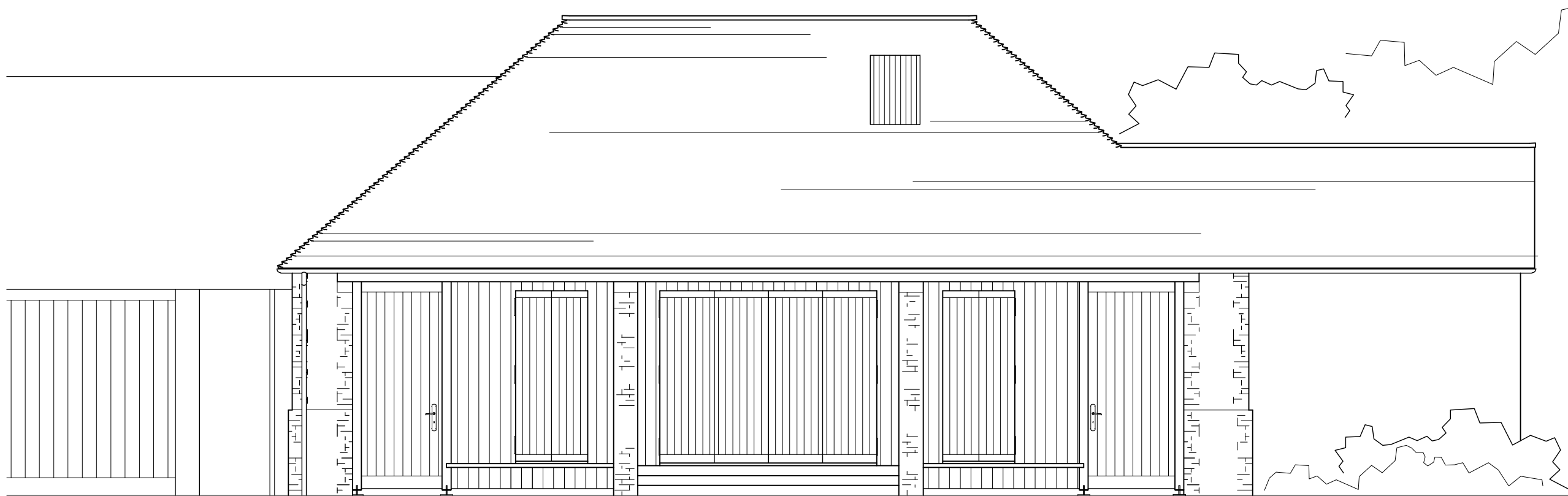
The Tractor Shed, Brighton Permaculture Trust Front ( east ) elevation, showing shutters closed
